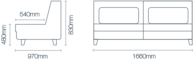
Chair: 630mm / 2.5 Seater: 1660mm / 3 Seater: 1960mm
