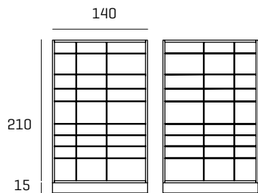
Q-Case 140x225 Lh-Rh . Dx-Sx
